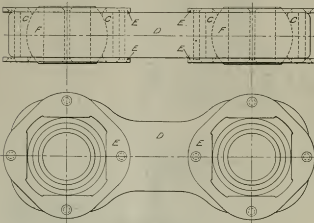
BALL JOINT DRAWBAR.
